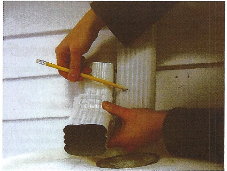
Figure 3. Marking the line where the downspout pipe will be cut and reconnected to the downspout elbow.
