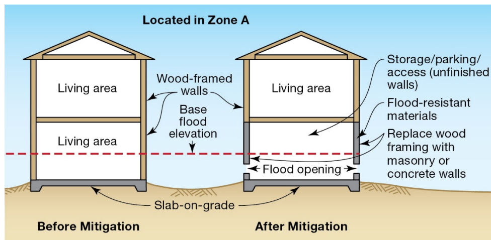
Figure 1. In Zone A, the floor below the BFE (left) can be modified to be compliant with NFIP criteria (right).
